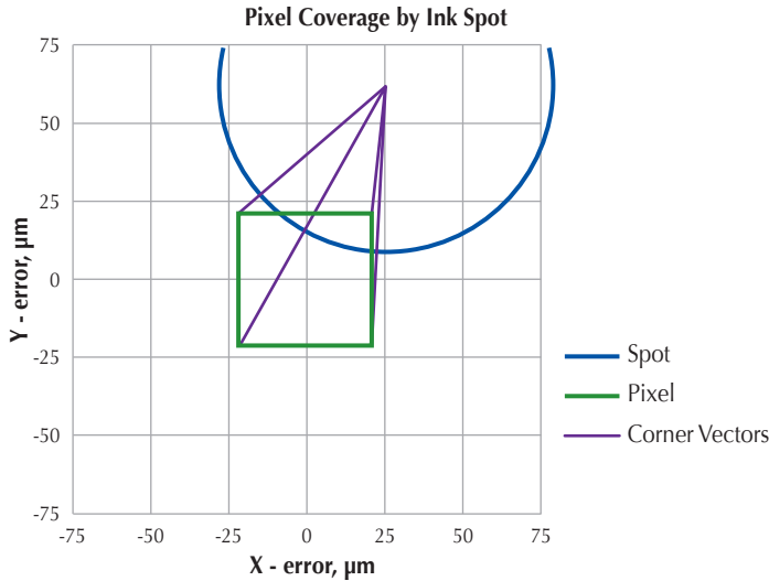
Figure 2. Ink spot, 106 \mu\text{m} in diameter, near a 600 \times 600 pixel
