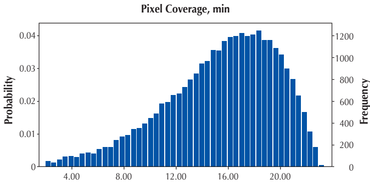
Figure 7. Pixel coverage at 1.0 mm standoff
