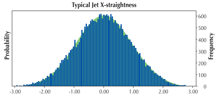
Figure 4. Typical jet X-straightness – normal distribution
