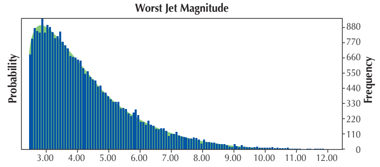
Figure 5. Worst jet X-straightness – Weibull distribution
