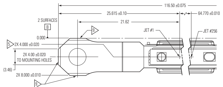
Figure 1. Sapphire interface control drawing with mechanical tolerances
