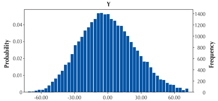
Figure 9. Y-ink drop position error distribution a 3 mm standoff
